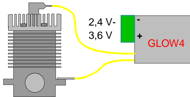
1-cylinder engine
